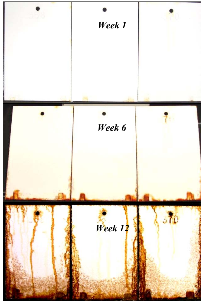
Figure 4-12 Photographs of System -9 Cyclic Corrosion Test
