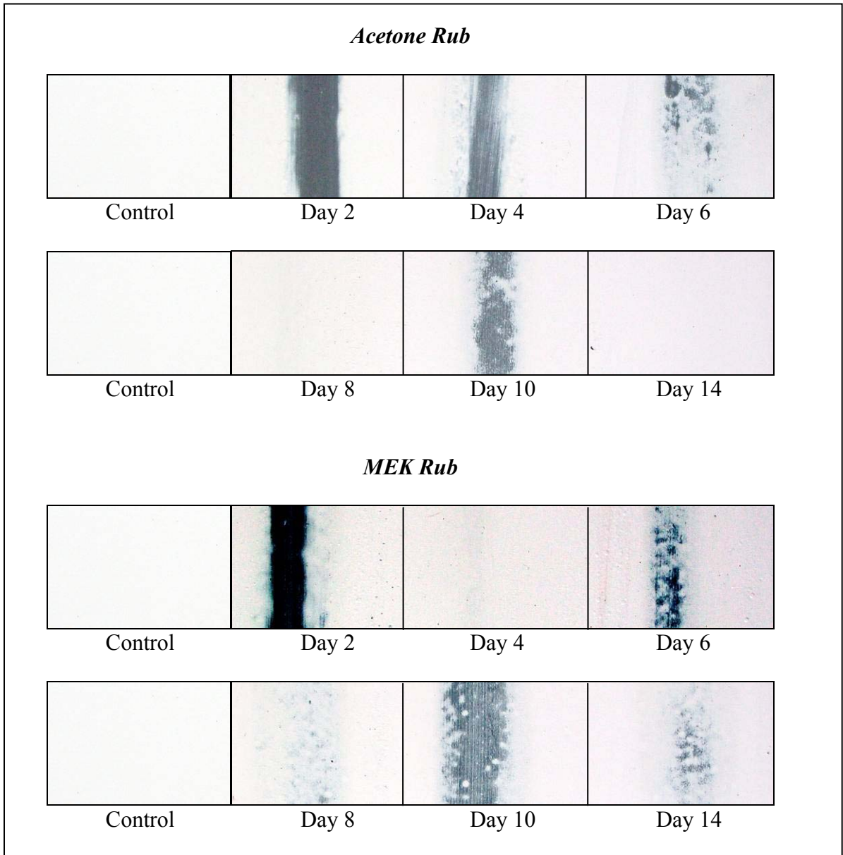
Figure 3-3 Photographs of System -4 Cure Time Evaluation
