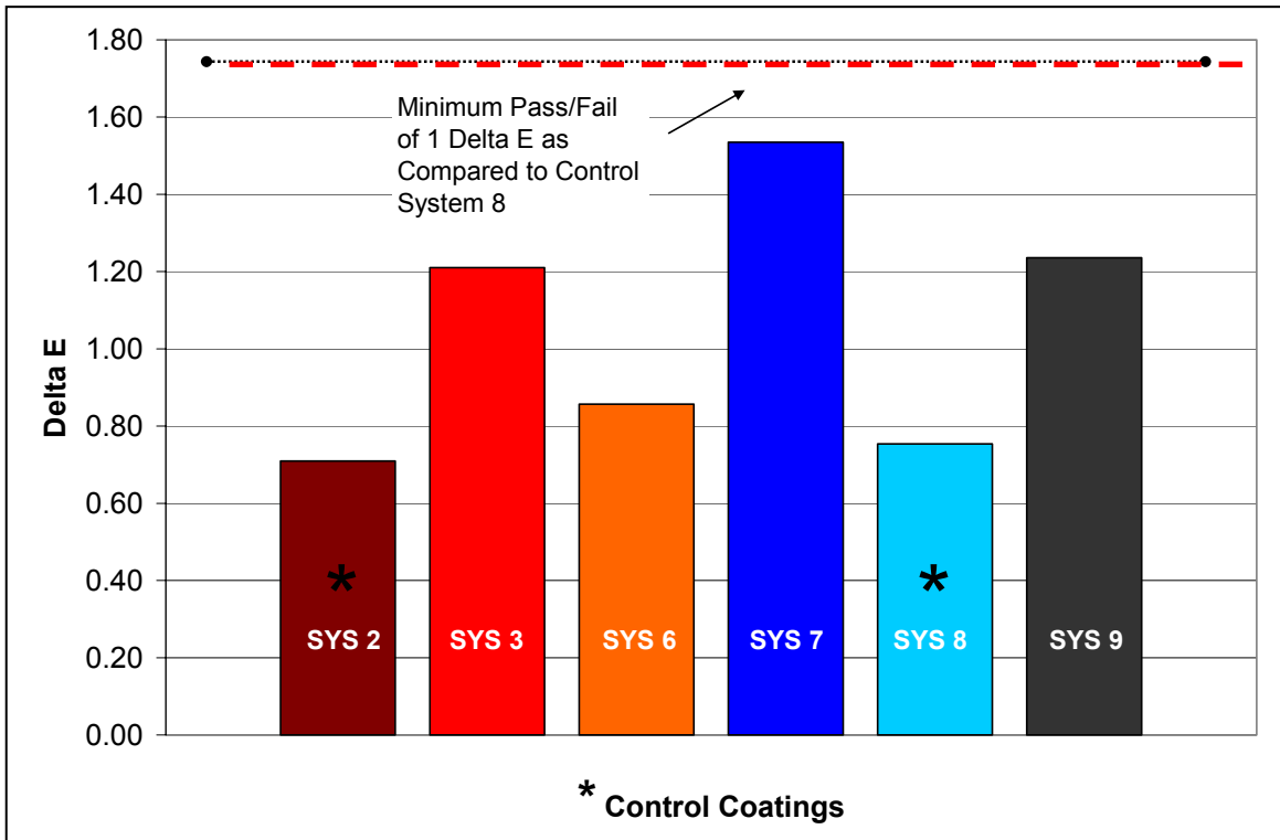
Figure 4-9 Delta E Color Difference – 1000 hour Exposure
