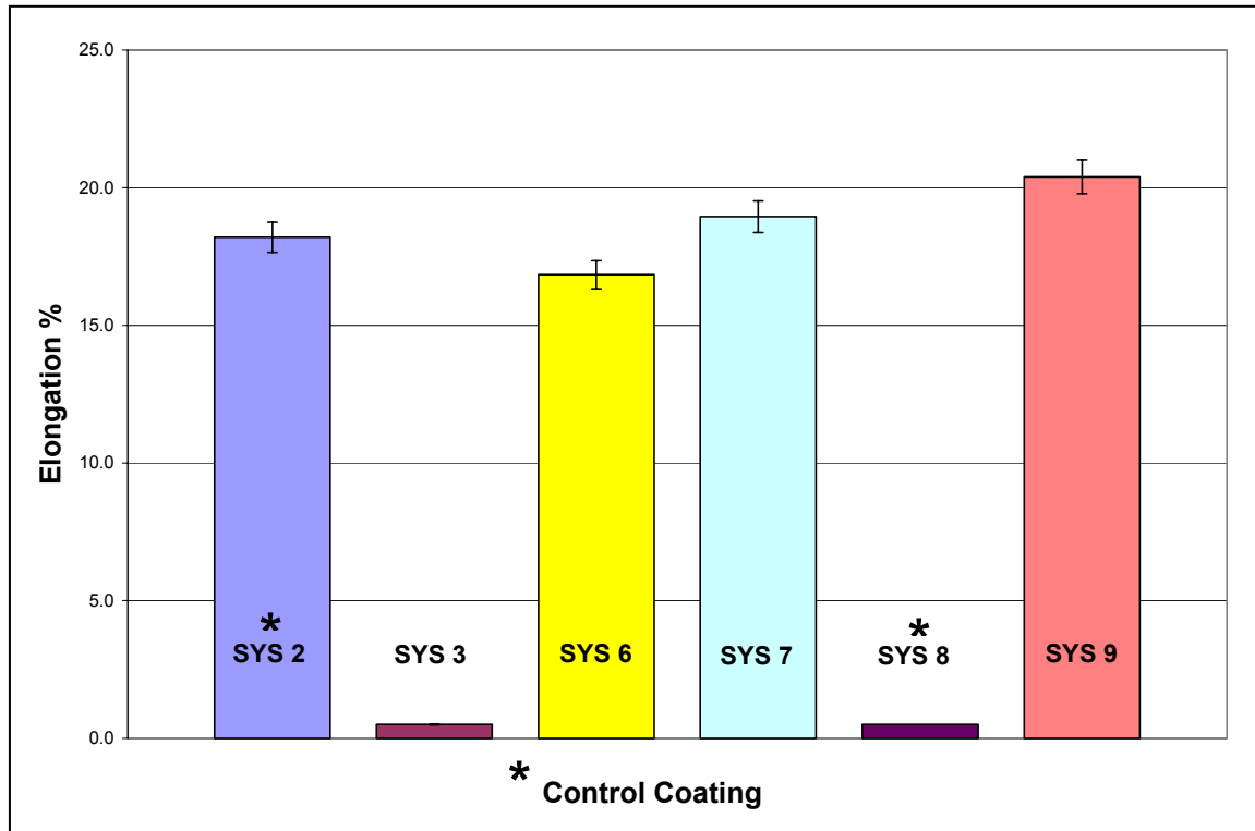
Figure 4-10 Coating Elongation from Mandrel Bend Test
