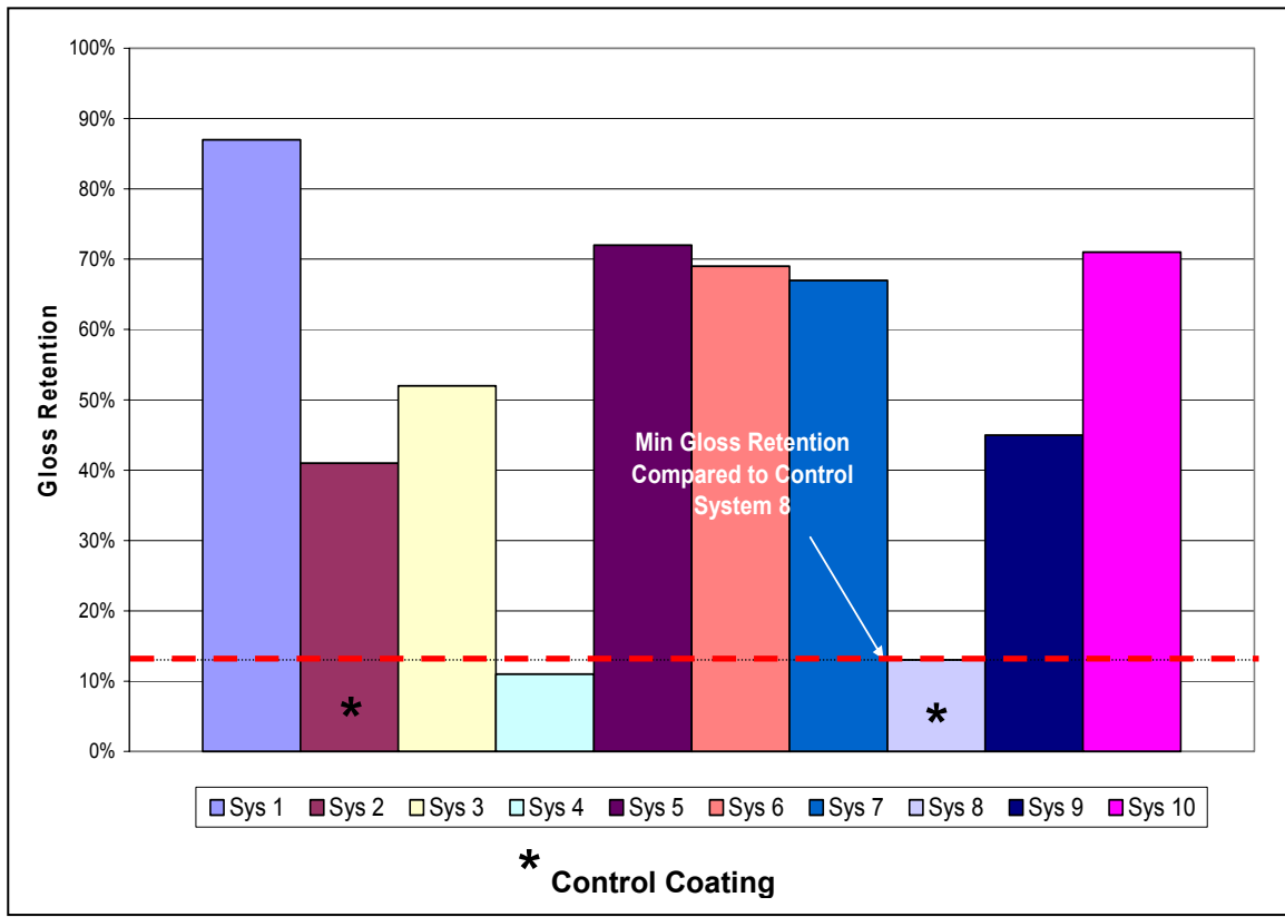
Figure 4-15 Results of 18-Month Marine Exposure Gloss Retention
