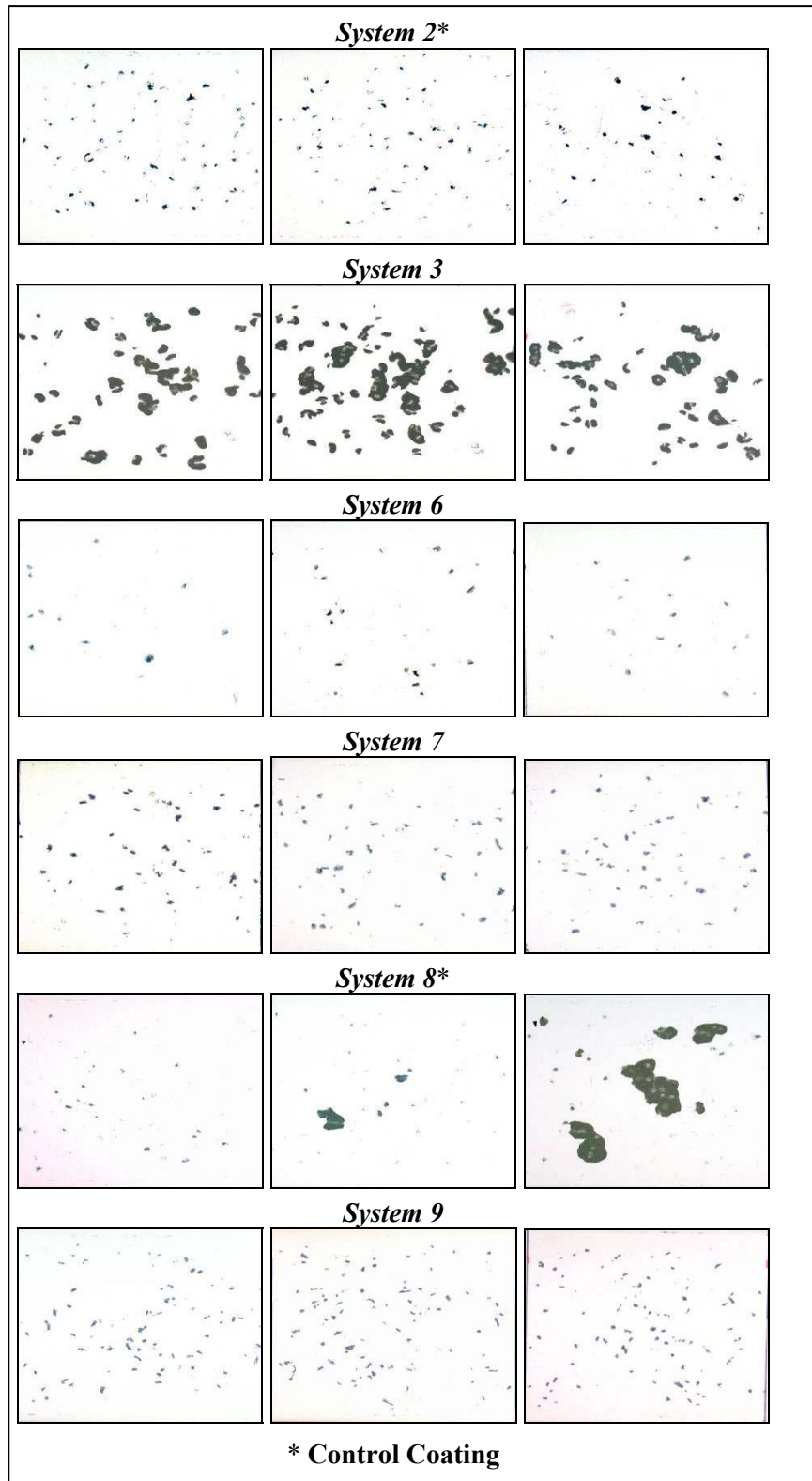
Figure 4-5 Gravelometer Chip Photographs
