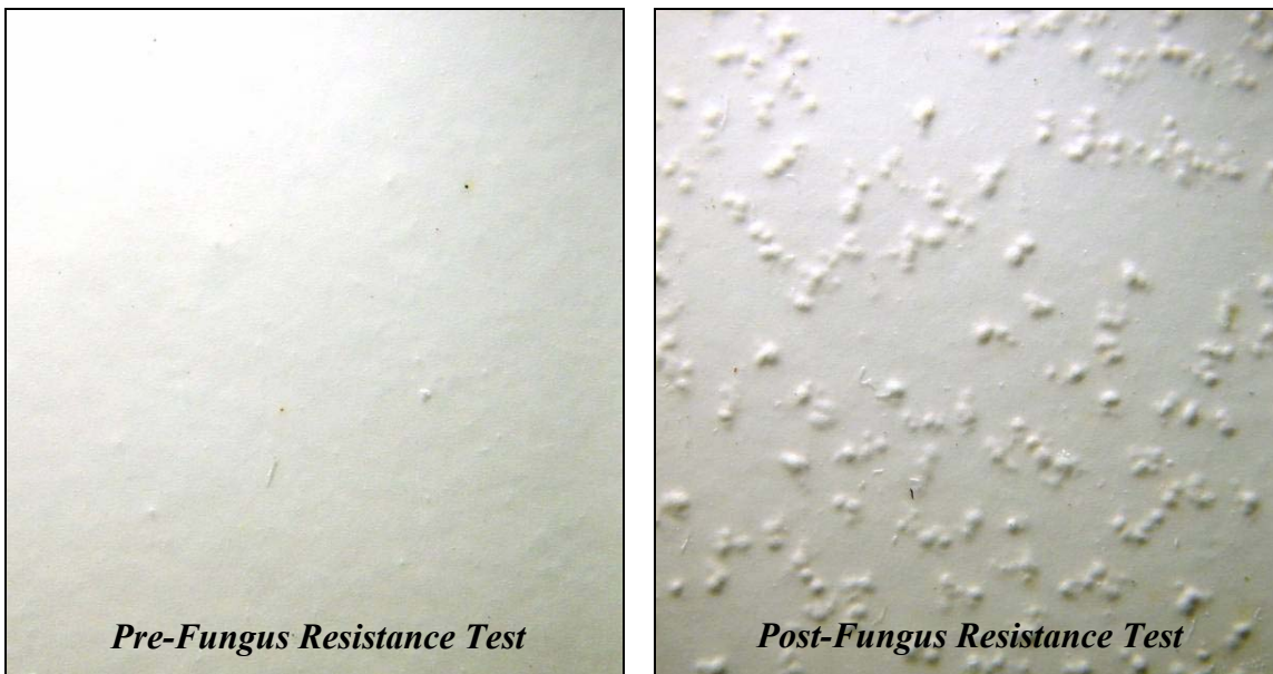
Figure 4-7 Photographs of Pre- and Post-Fungus Resistance Test for System -9
