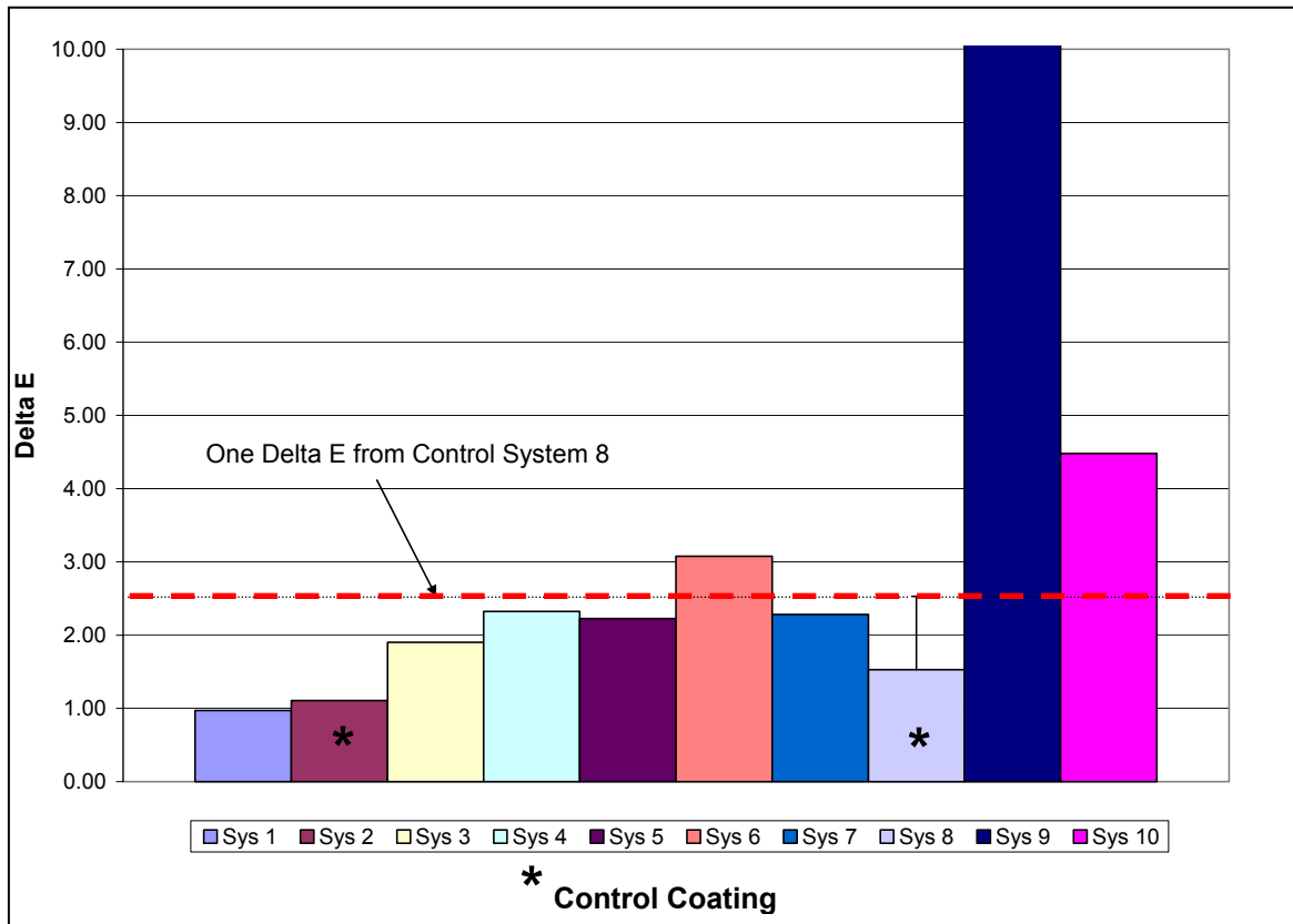
Figure 5-4 Results of Color Retention from SSC Field Testing
