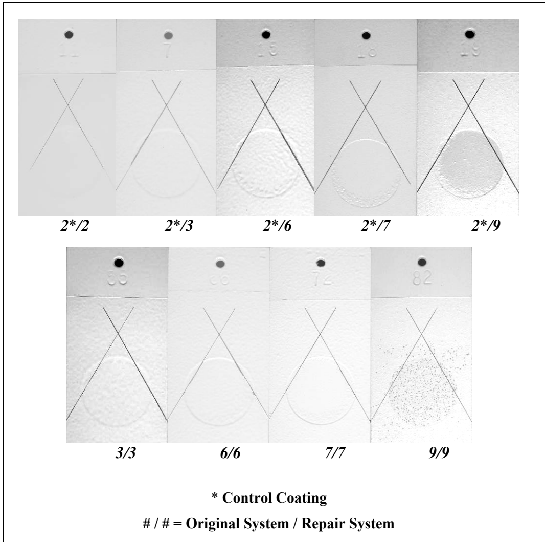
Figure 4-2 Photographs of Repairability Results
