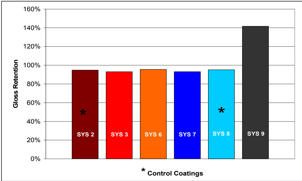
Figure 4-8 Gloss Retention of Accelerated Weathering Coatings – 1000 hour Exposure
