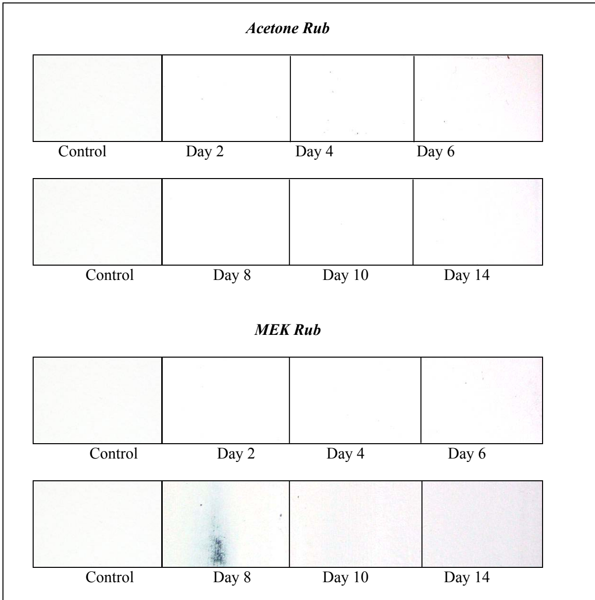
Figure 3-5 Photographs of System -5 Cure Time Evaluation
