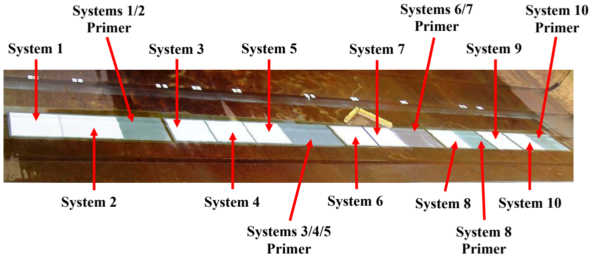
Figure 5-2 Field Coating Application Sections
