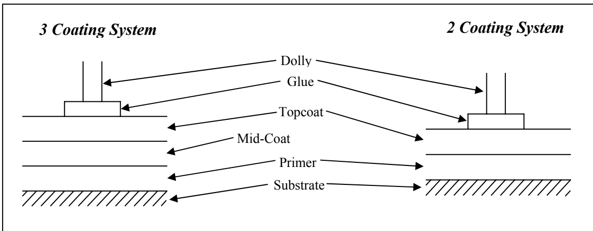
Figure 3-7 Coating System Interfaces
