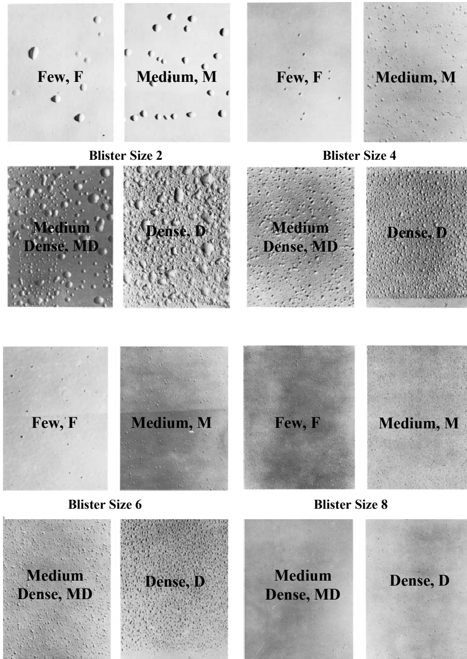
Figure 4-17 Photographs of ASTM D 714 Blister Reference
