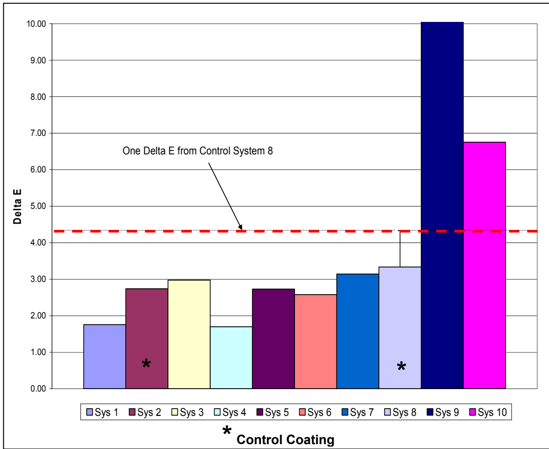
Figure 4-16 18-Month Marine Exposure Color Change Results
