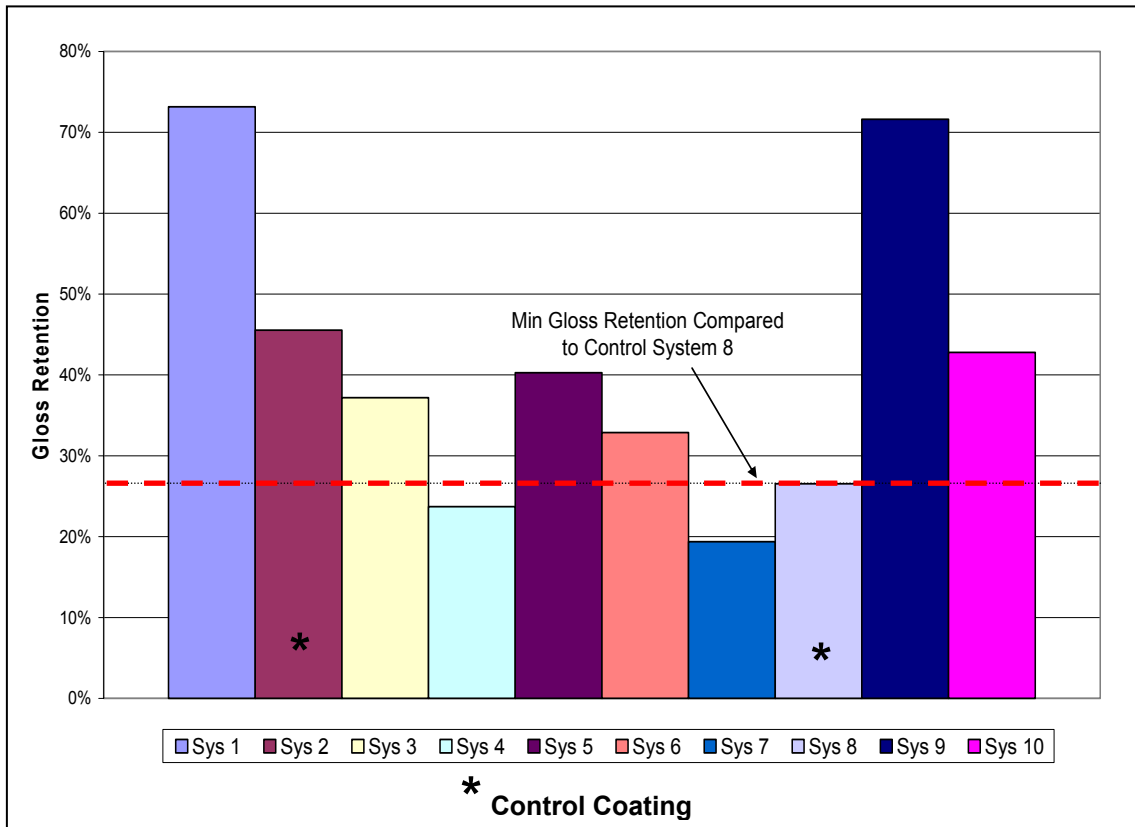
Figure 5-3 Results of Gloss Retention from SSC Field Testing
