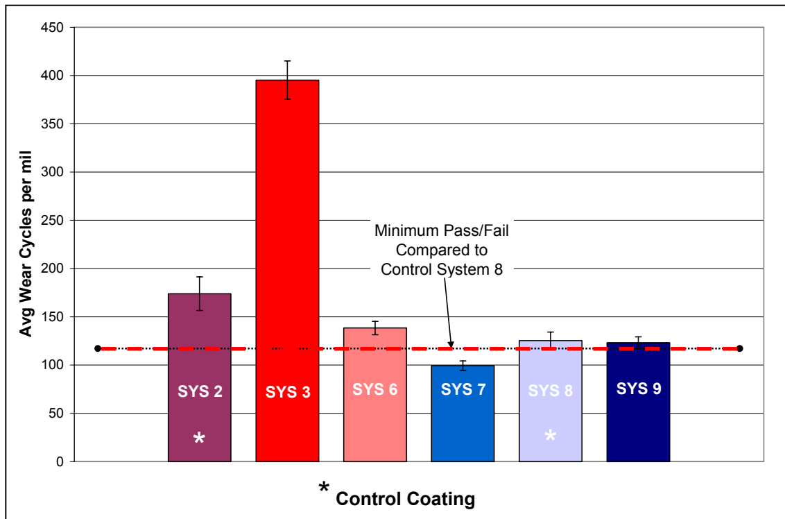
Figure 4-3 Taber Abrasion Wear Cycles per mil
