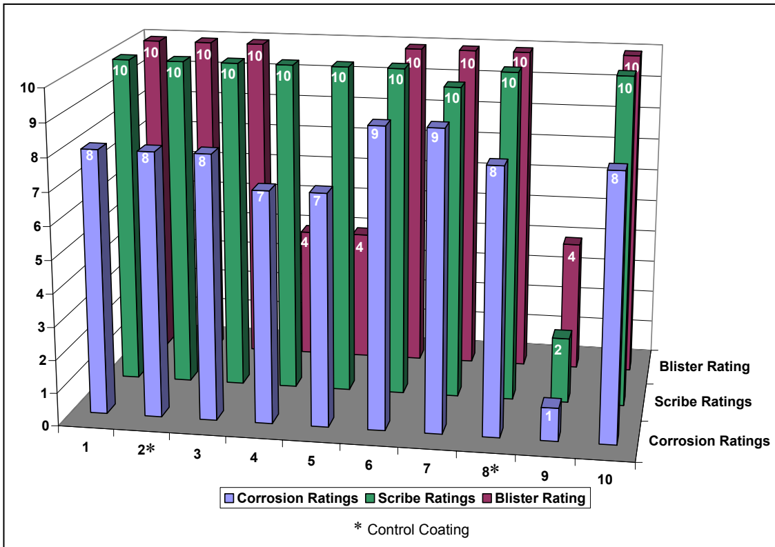
Figure 4-18 18-Month Beach Exposure Corrosion Ratings
