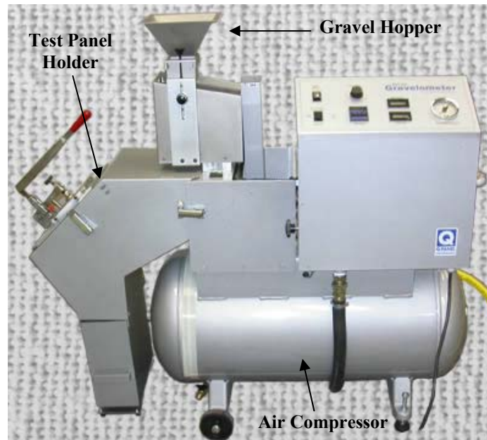
Figure 4-3 Gravelometer Apparatus
