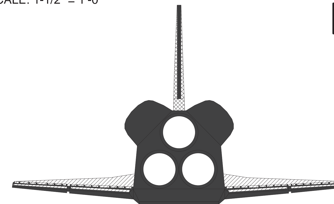
HRSI/ LRSI = HIGH/ LOW TEMPERATURE REUSABLE SURFACE INSULATION DETAIL SCALE: 1-1/2" = 1'-0"
