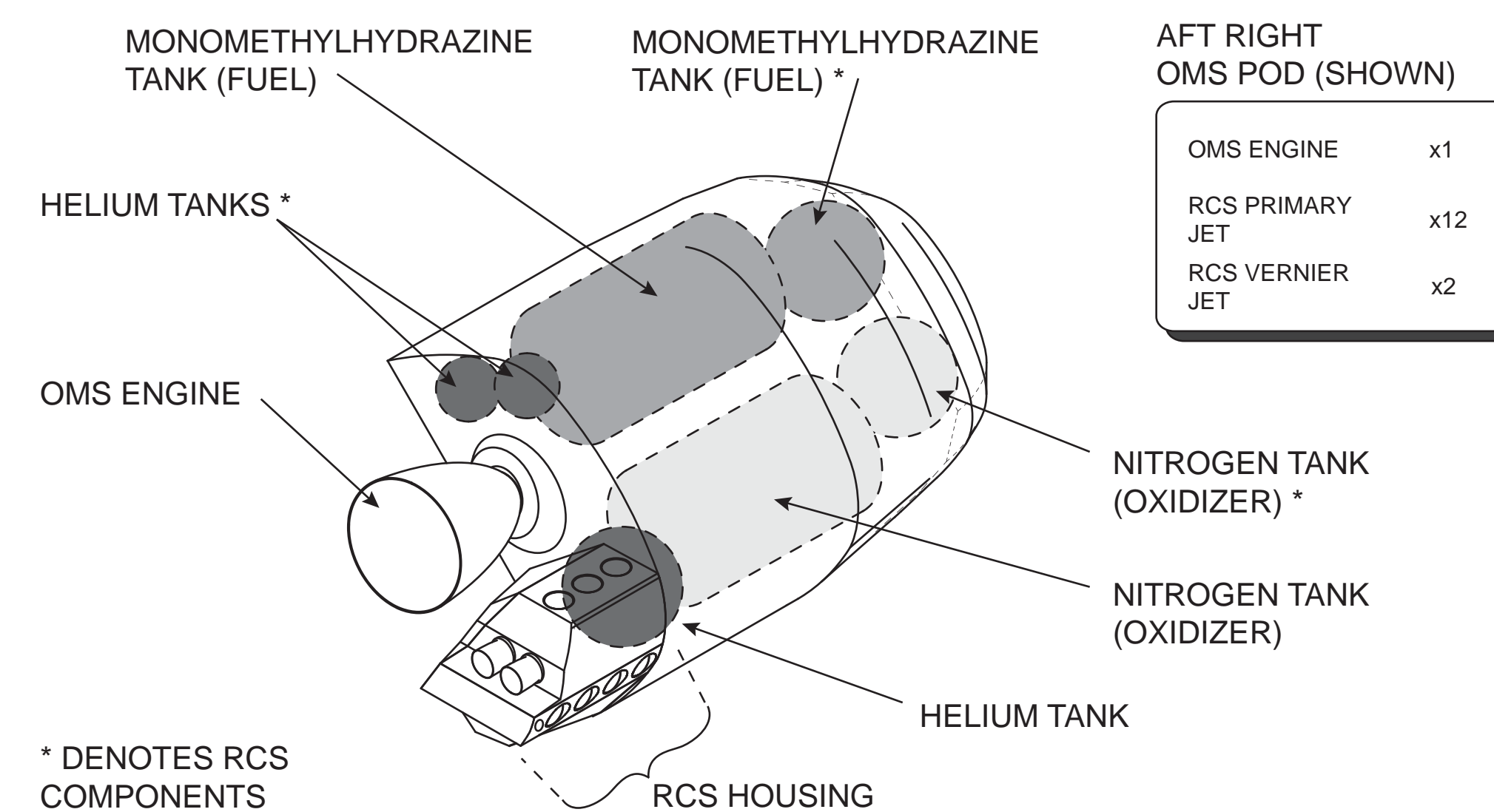
ORBITAL MANEUVERING SYTEM (OMS) & AFT REACTION CONTROL SYSTEM (RCS)
