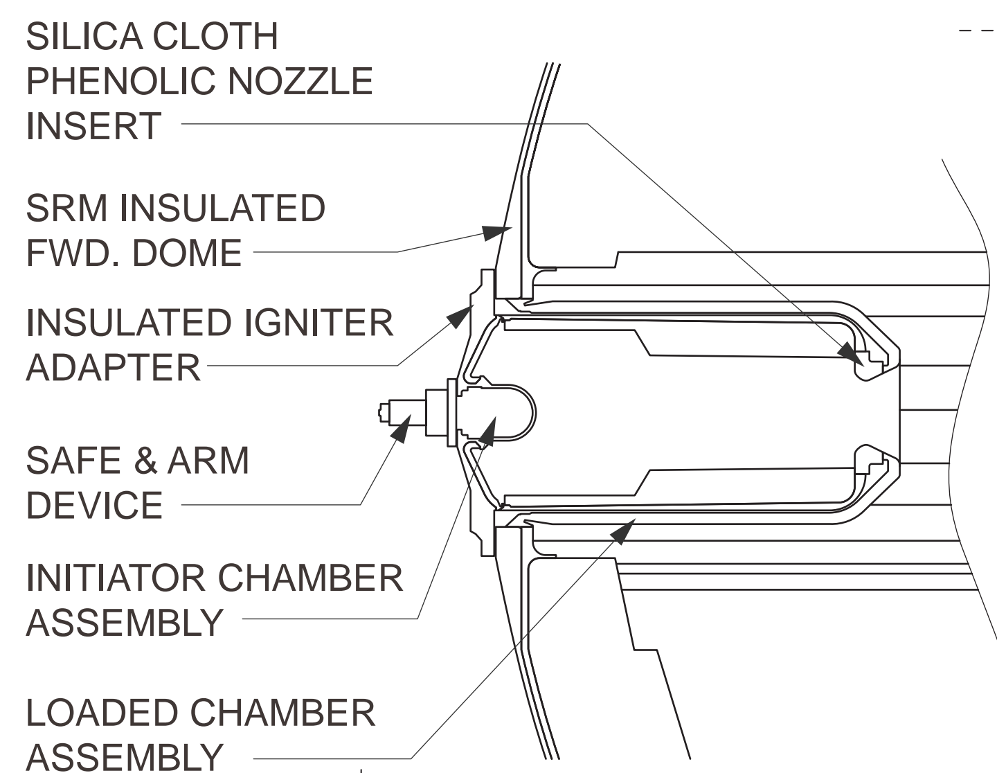
SRB IGNITOR DETAIL SCALE: 1" = 1'-0"
