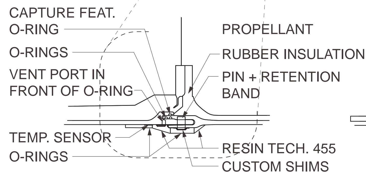
FIELD WELD JOINT SCALE: 2" = 1'-0"
