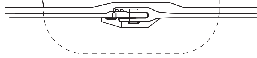
FACTORY WELD JOINT SCALE: 2" = 1'-0"
