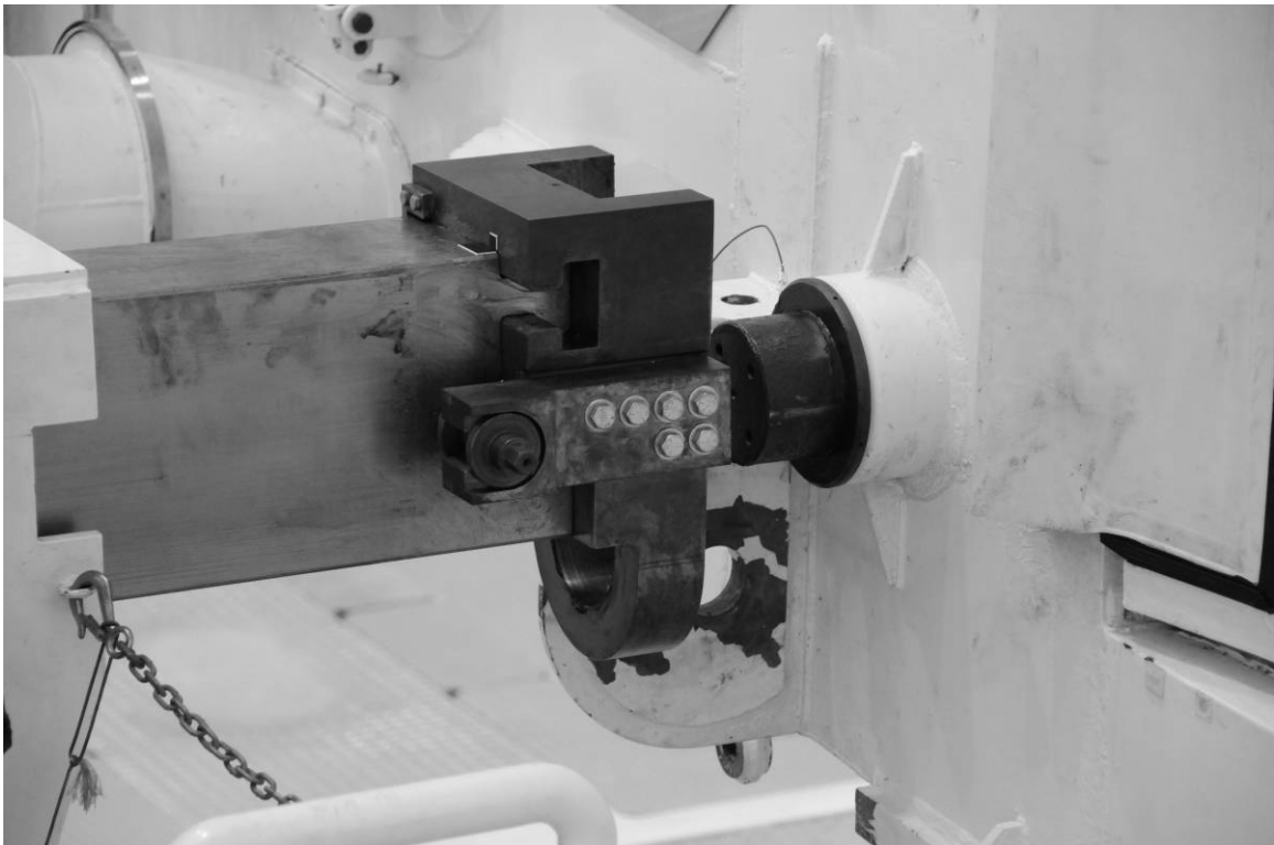
Figure A-19. Detail view showing a U-saddle being retracted, April 13, 2010. Source: Penny Rogo Bailes.
