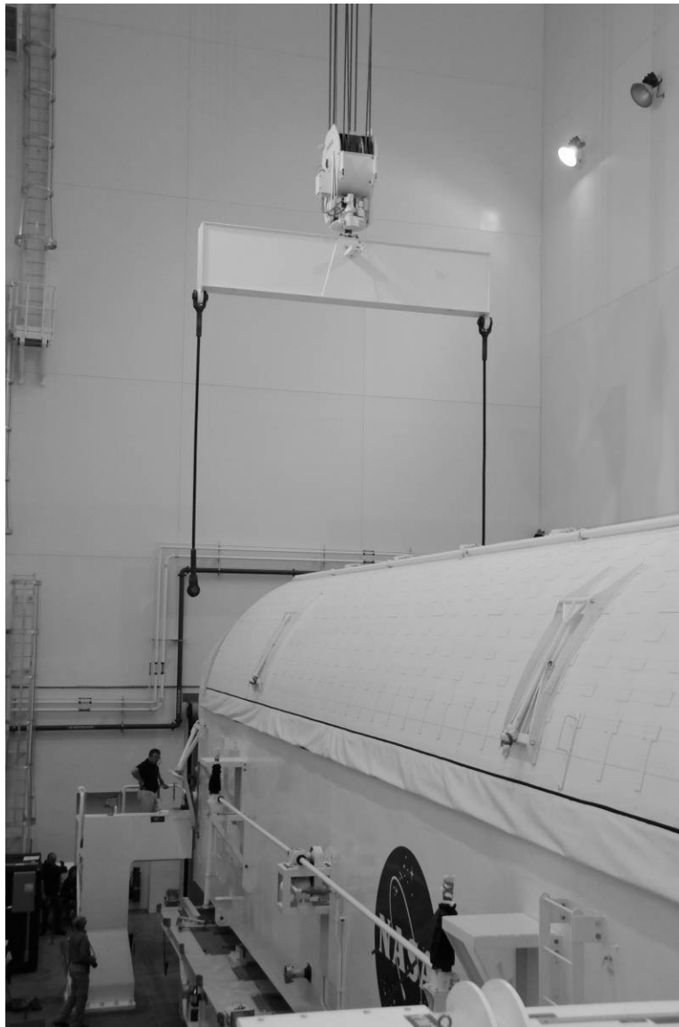
Figure A-12. Detail view showing a lifting beam and slings being lowered for attachment to forward lug retainers, April 13, 2010. Source: Penny Rogo Bailes.
