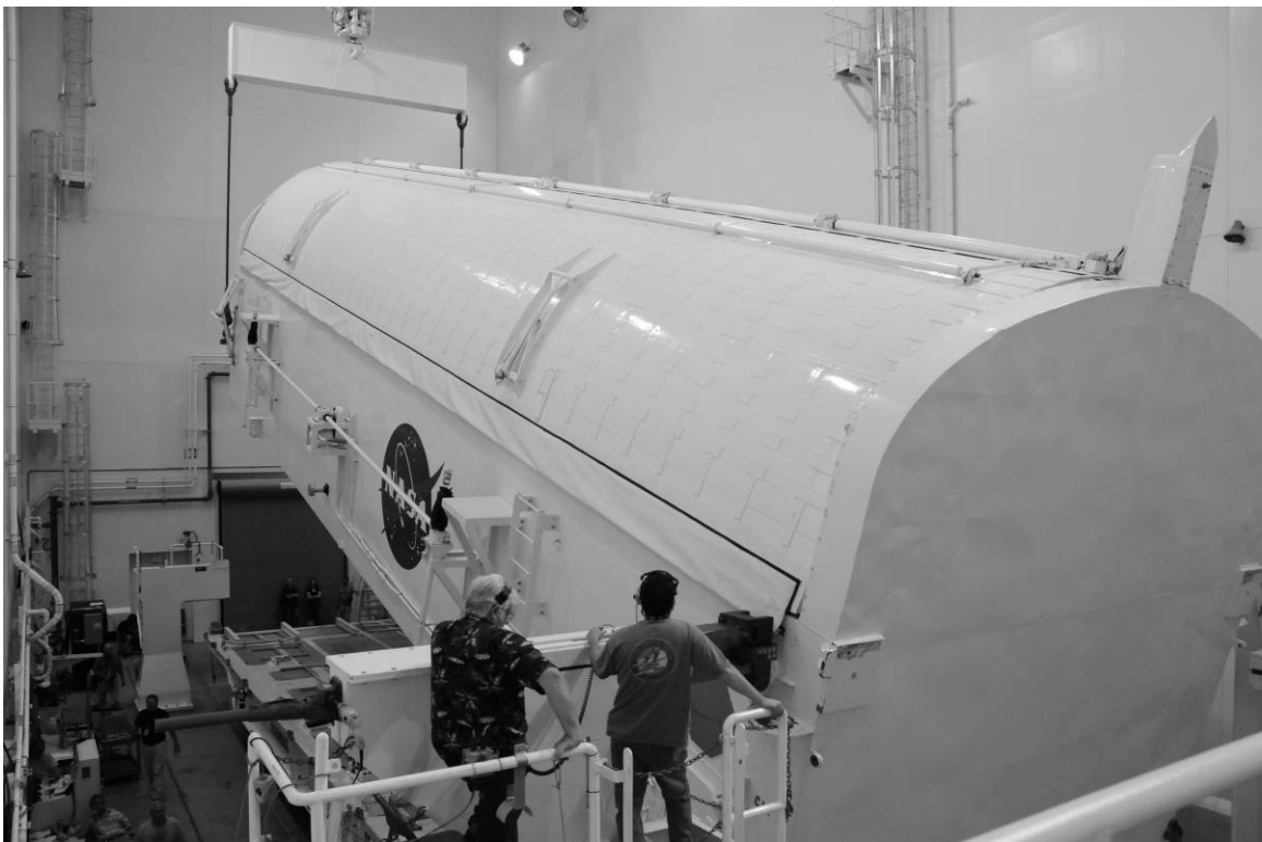
Figure A-15. View showing the rotation process of the payload canister approximately one-third complete, April 13, 2010. Source: Penny Rogo Bailes.
