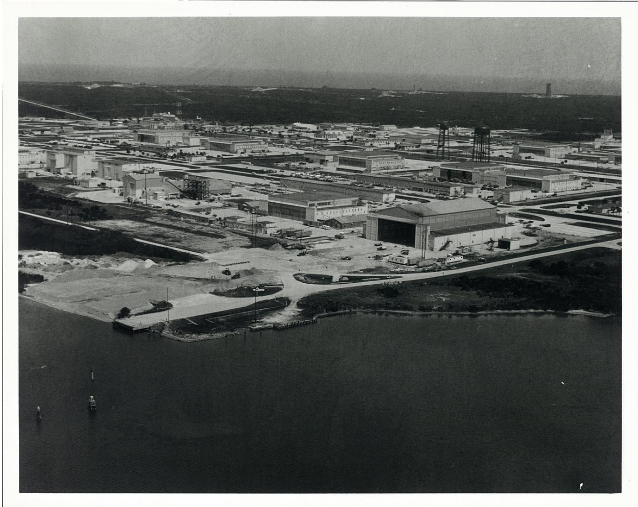
Figure 5. This 1978 aerial photograph of the construction at the Hangar AF site shows the condition of Hangar AF and the High Pressure Gas Building at the beginning of site grading and other preparations for the Space Shuttle Program. (Courtesy of KSC, Image 108-KSC-378C-203/3).
