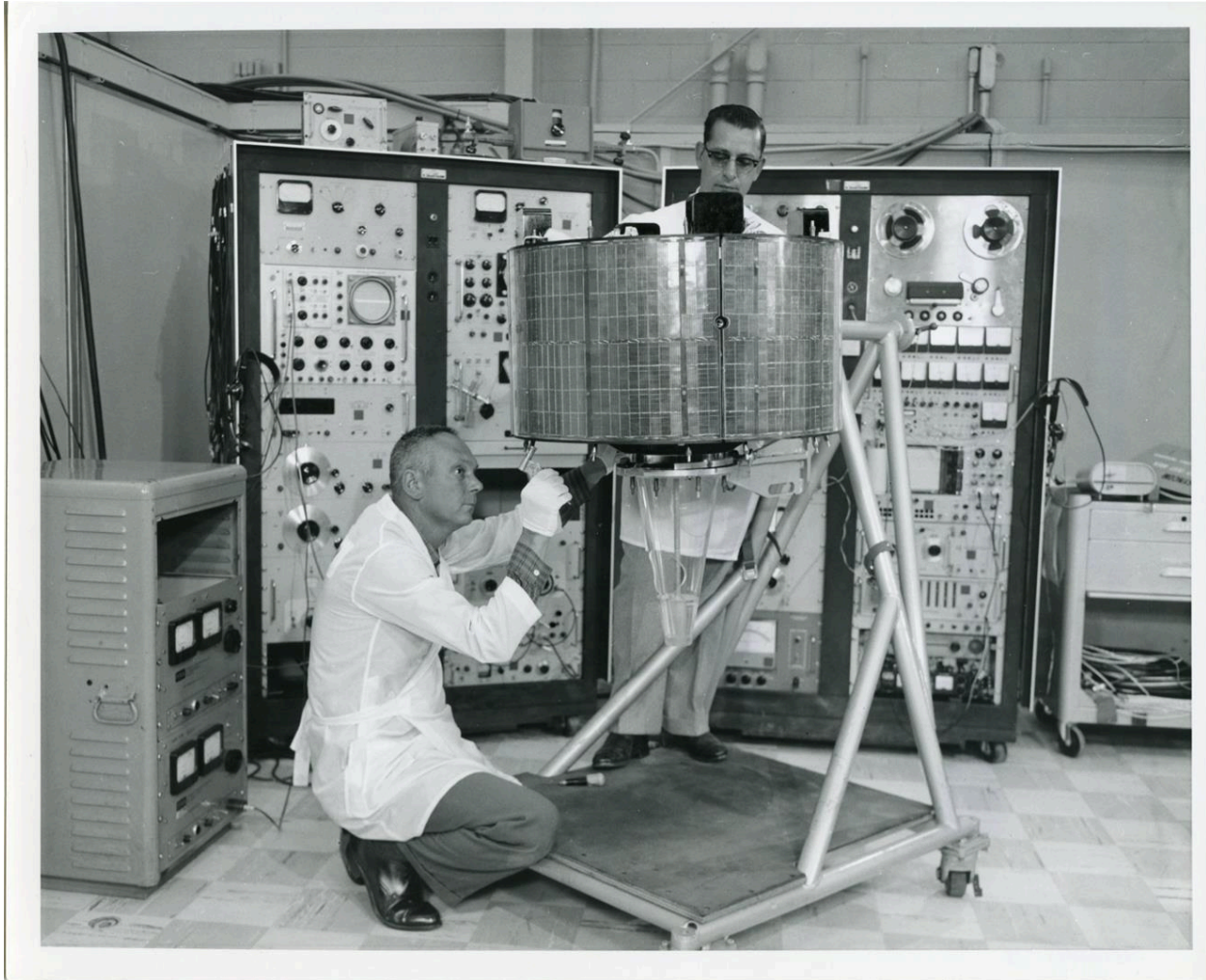
Figure 12. Hughes Aircraft Co. engineers conduct final checkout of Syncom 1 satellite in Hangar AE high bay prior to mating to Delta launch vehicle. (Courtesy of Kennedy Space Center Archives, Image 63-Syncom-20).
