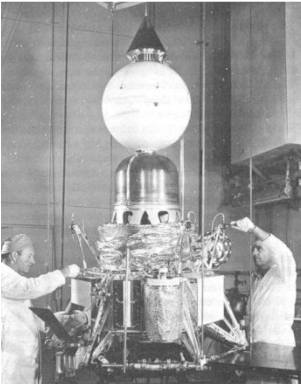
Figure 9. Technicians make final adjustments to the Ranger 3 Spacecraft at Hangar AE. (Source: "Lunar Impact: A History of Project Ranger," NASA History Division, 2006.)
