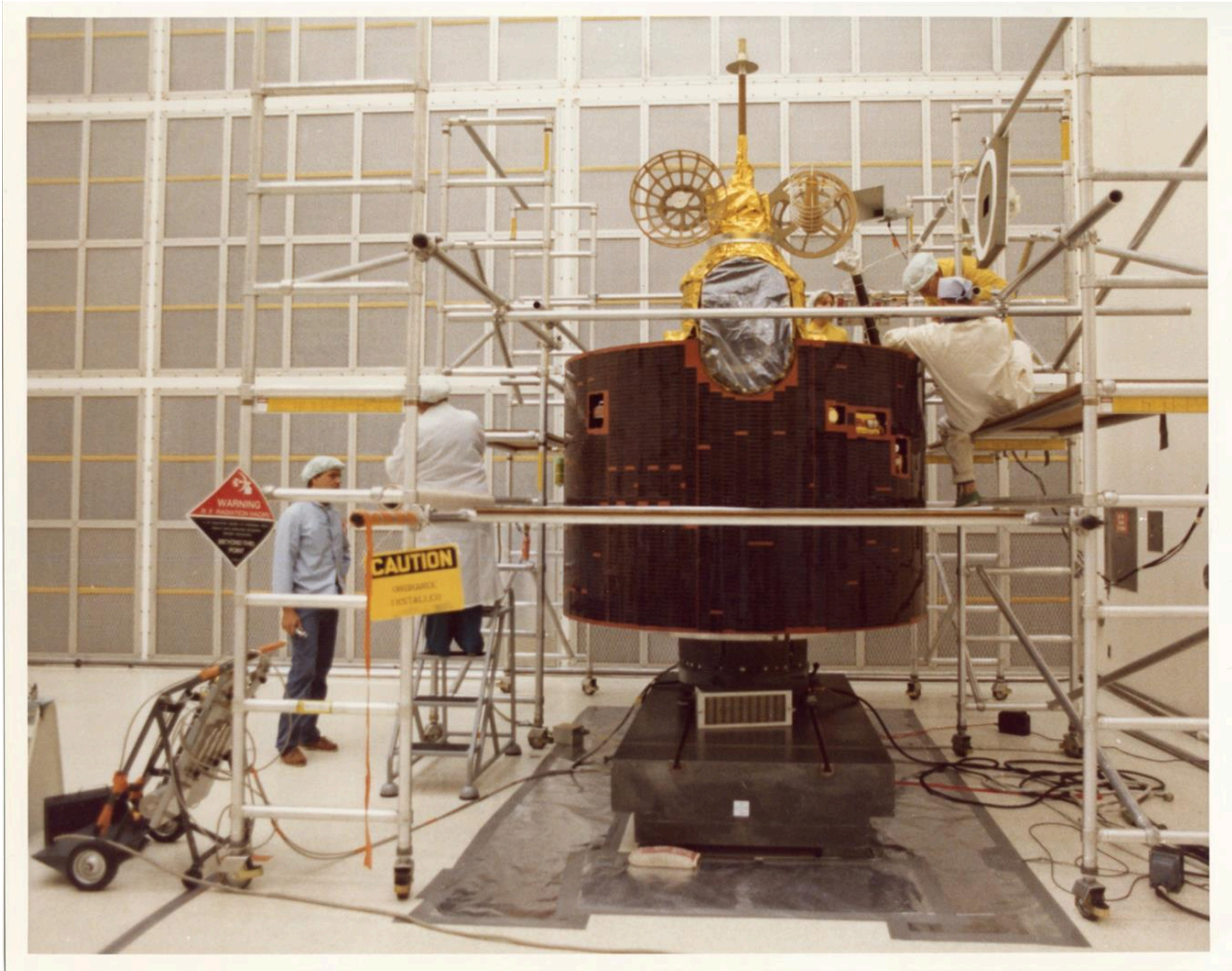
Figure 13. Engineers check out the GOES-6 satellite in Hangar AE high bay, 1983. (Courtesy of Kennedy Space Center Archives, Image 102-KSC-383C-1019-5).
