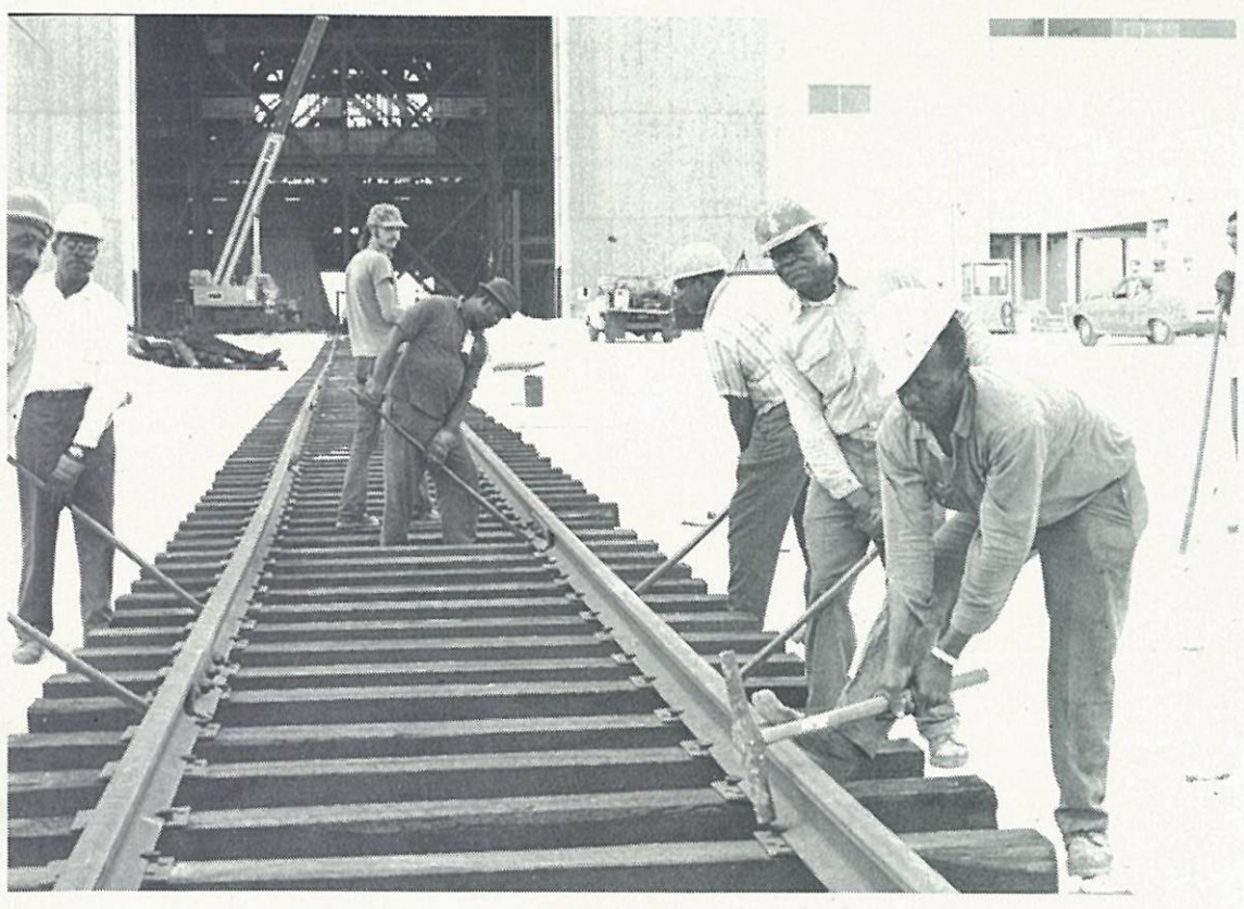
Figure A-8. Construction of the railroad spur in the VAB, May 1977. Source: Spaceport News , May 27, 1977, page 1.
