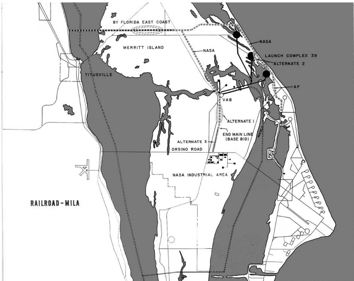
Figure A-3. Chart showing initial plan of the railroad system, August 21, 1963. Source: Kennedy Institutional Image Facility, KSC-63C-2574.
