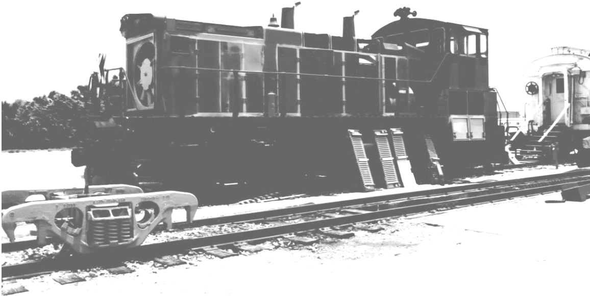
Figure A-15. View of one of the General Motors locomotives as purchased in July 1984. Source: John F. Kennedy Space Center Transportation Office, 114-KSC-385C-2658.7.
