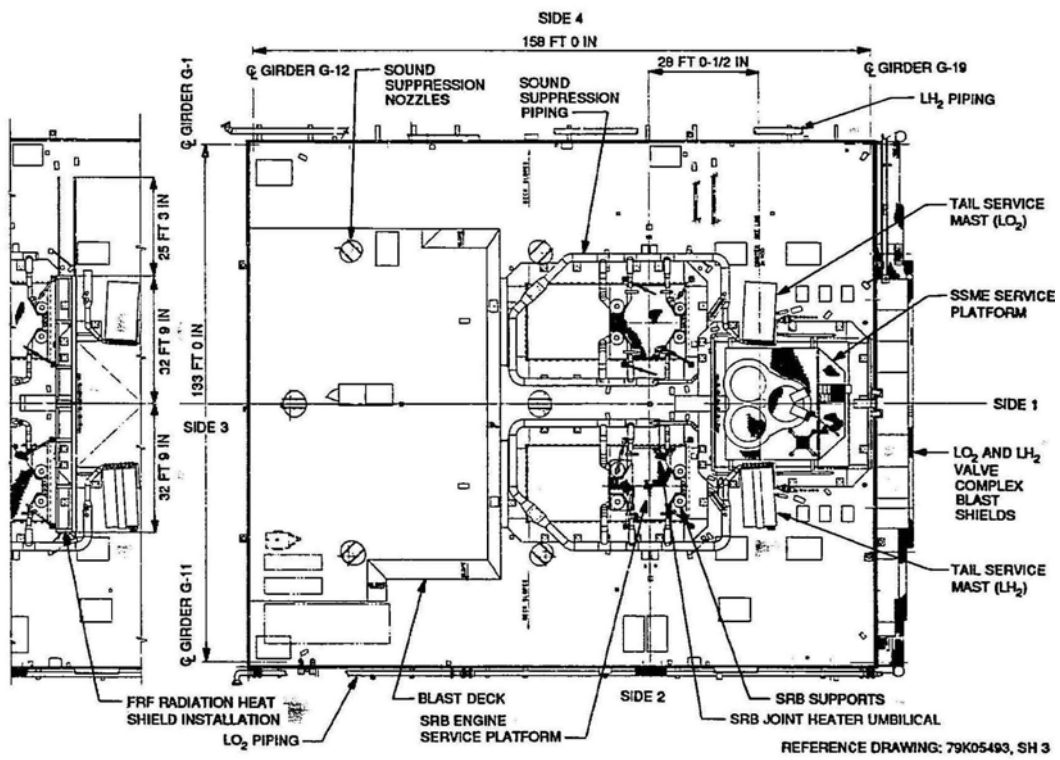
Figure 10. Diagram of the MLP's 0 Level. Source: NASA KSC. Space Shuttle Launch Support Equipment Data Handbook , March 30, 1993.
